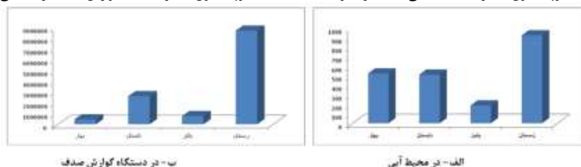
Figure 5: Comparison of total annual zooplankton cells in the two aquatic environment and gastrointestinal tract of A. cygnea in Anzali Lagoon in different seasons
