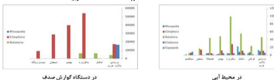
Figure 5: Comparison of total annual zooplankton cells in the two aquatic environment and gastrointestinal tract of A. cygnea in Anzali Lagoon in different seasons
