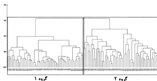
Figure 6: Cluster analysis of zooplankton at sampling stations.
