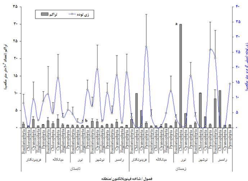
Figure 2: Density and biomass of phytoplankton's different divisions among of different seasons and depths in the Caspian Sea.
