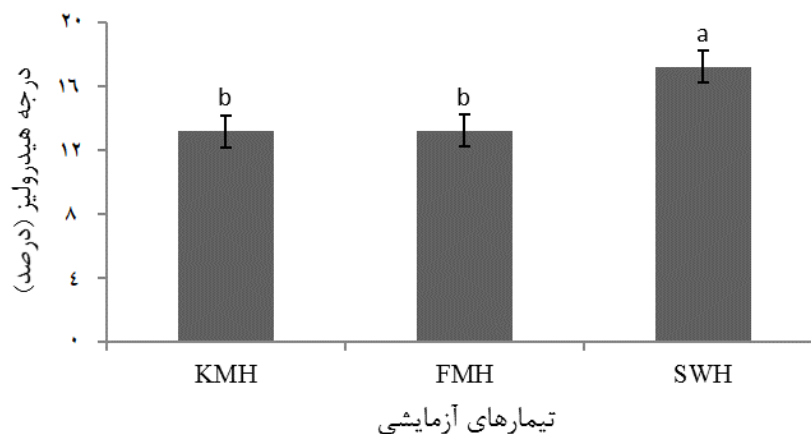
Figure 1: Degree of Hydrolysis of Kilka's meat (KMH), fishmeal (FMH) and stickwater (SWH) protein hydrolysates
