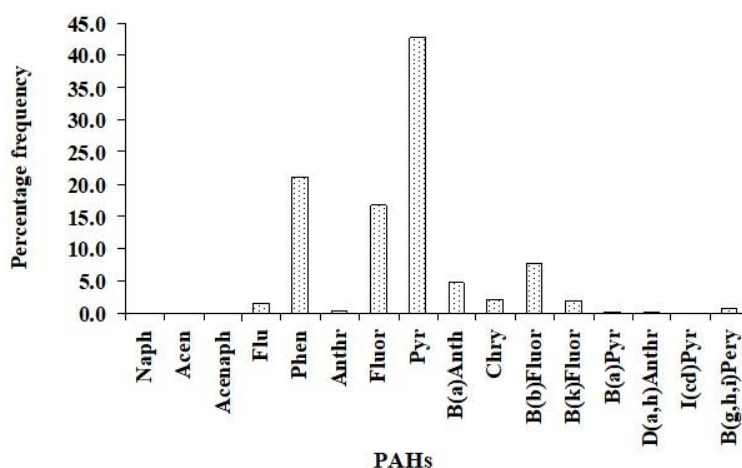
Figure 2: Percentage frequency of 16PAHs of sediments in the southern basin of Caspian Sea (2018-2019)
